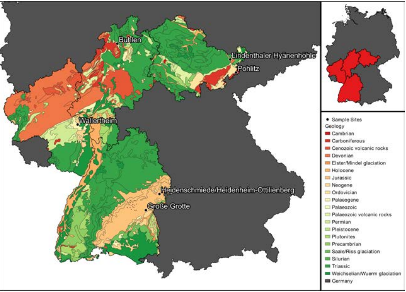
Fig. 2 Geology around the sampled Late Neanderthal sites in central and southern Germany as well as the location of the woolly rhino from Pohlitz, which was radiocarbon dated additionally (modified after GK2000).
