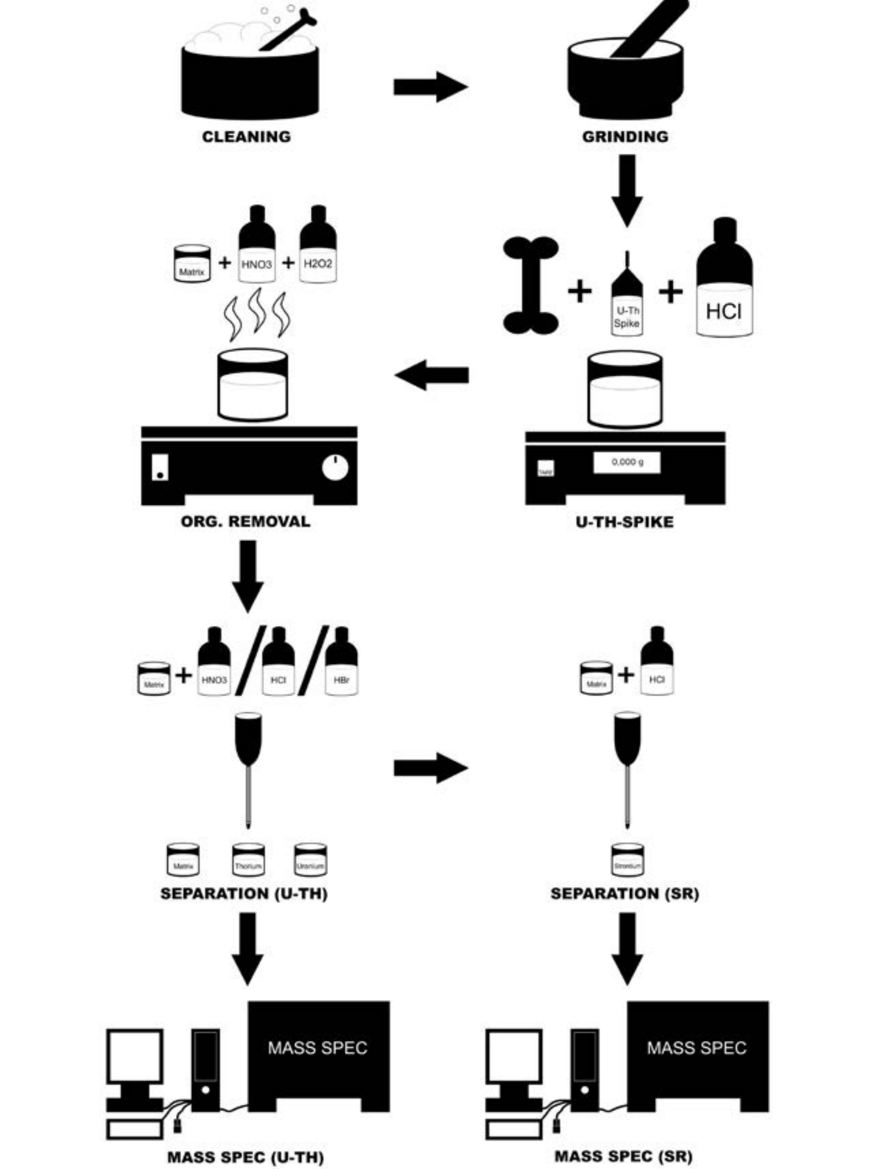
Fig. 3 Applied methods for strontium and uranium-thorium isotope analysis.
